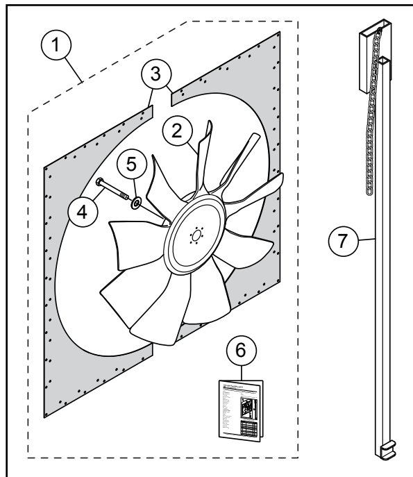
Figure 1. Fan Replacement Parts
