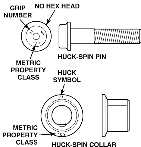
Figure 1 — Huck-Spin® Pin and Collar
